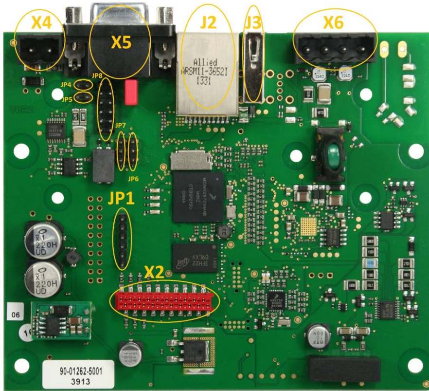
Figure 3 EVSE board with marked connectors
