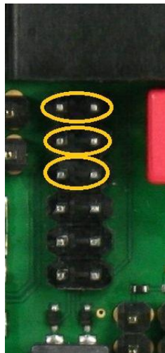
Figure 8 JP8 in RS232 MODE
