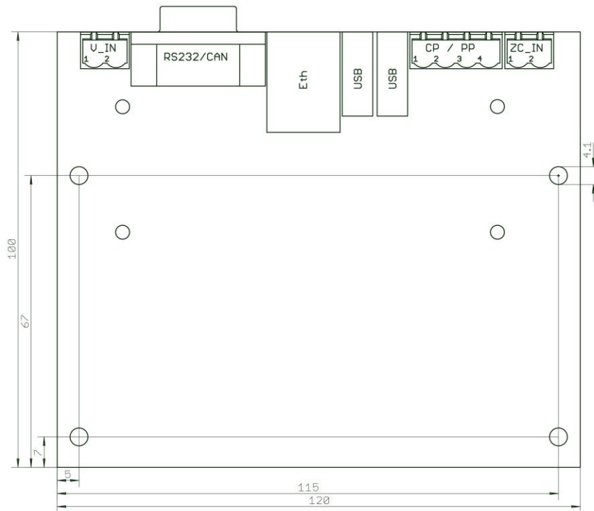
Figure 1 Mechanical drawing of EVAcharge SE including connectors
