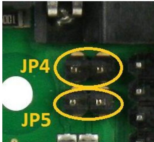
Figure 9 CAN termination jumpers JP4 and JP5
