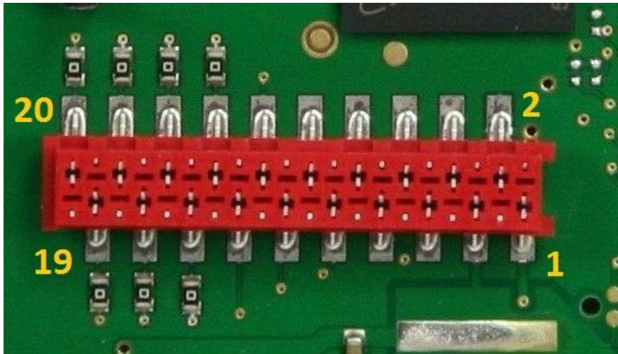
Figure 11 Daughter board connector
