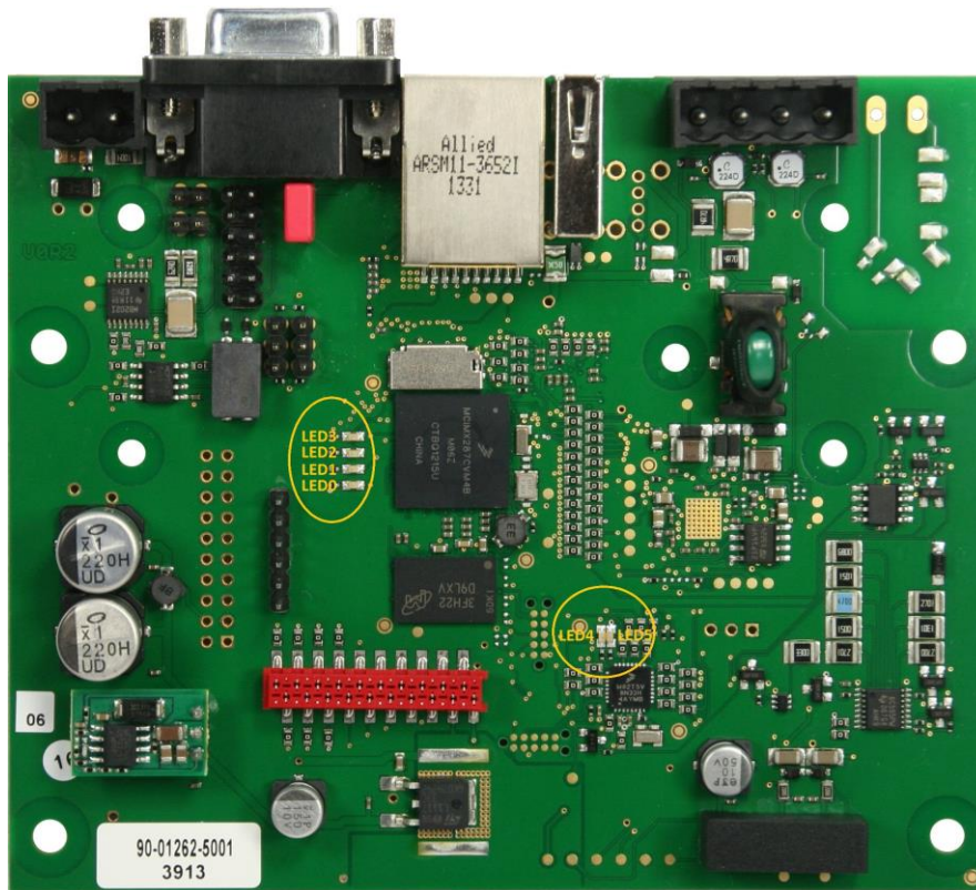
Figure 2 LEDs on EVSE
