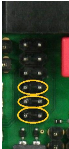
Figure 7 JP8 in CAN MODE
