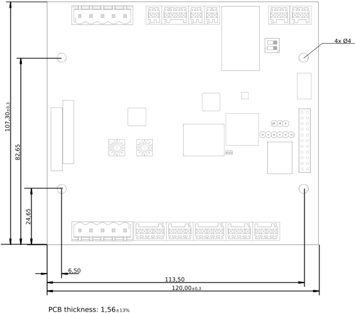
Figure 1: Mechanical drawing of Charge Control C, dimensions in mm
